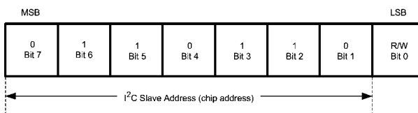
FIGURE 5. Chip Address
