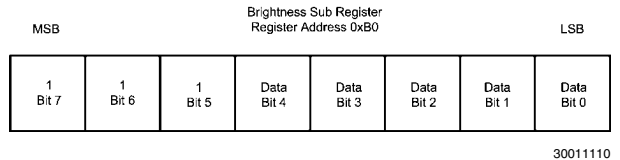
FIGURE 9. Brightness SUB Register Description
