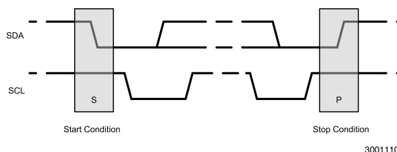
FIGURE 4. Start and Stop Sequences
