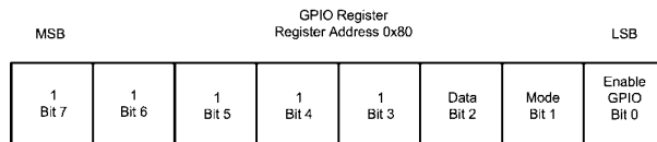
FIGURE 11. GPIO Register Description
