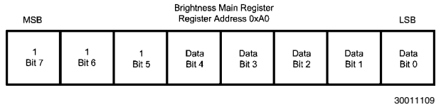
FIGURE 8. Brightness MAIN Register Description
